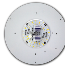
SL18-AC120RT-W-M802PL 24W, 1980LM, 3000K
