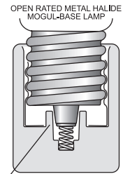
Inner wall in lampholder allows only Open Rated Lamp use.
