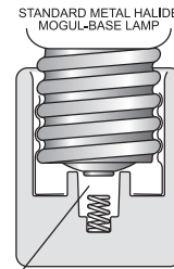
Lamp contact does not make contact with the lampholder.
