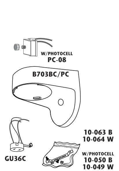
ASSEMBLY S313-G
