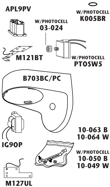
ASSEMBLY S313-M
