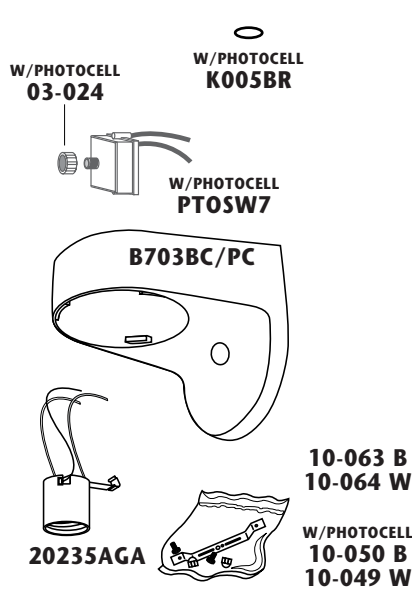
ASSEMBLY S313-I60
