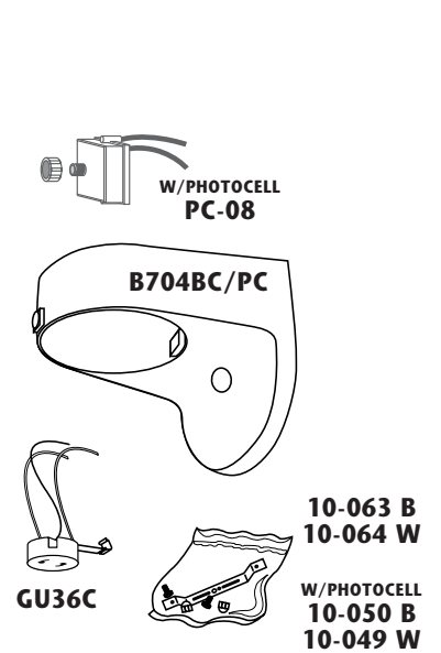
ASSEMBLY S314-G
