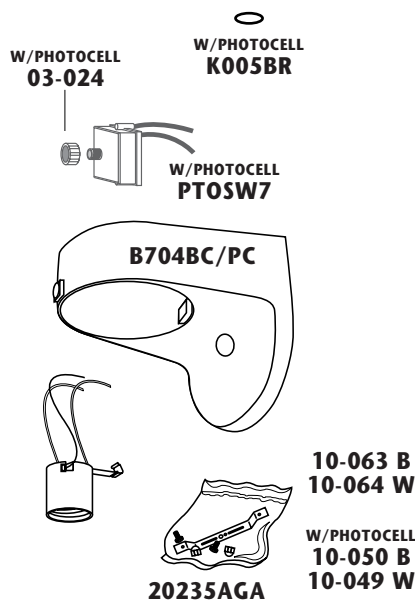
ASSEMBLY S314-I60
